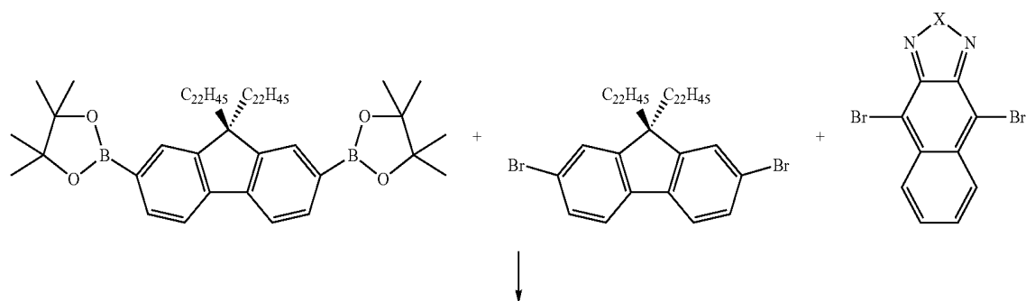
Scheme 2. General synthesis of NTD and NSeD containing polymers
