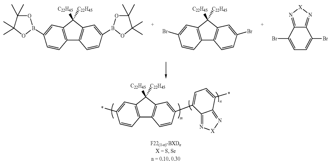
Scheme 1. General synthesis of BTD and BSeD containing polymers
