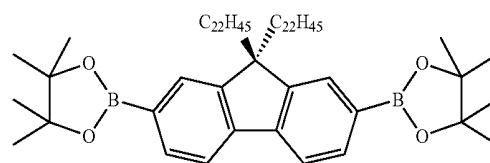
F22-diborate
